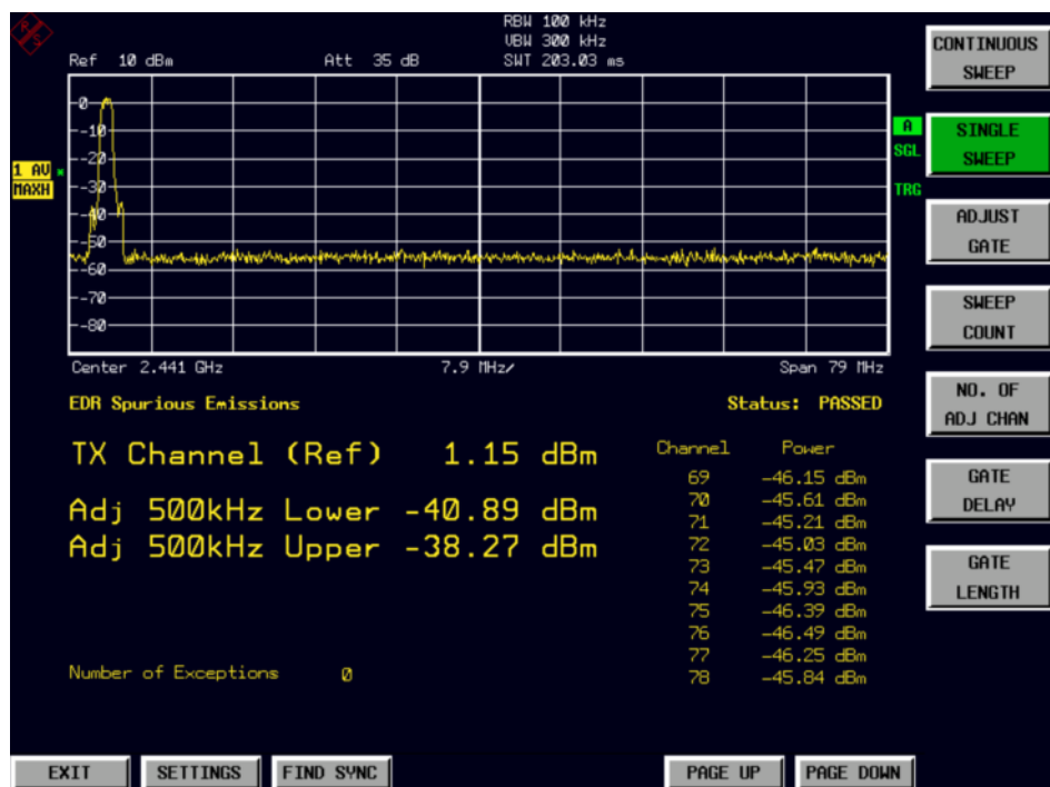
Bild 3-11 In-Band Spurious Emissions (EDR)
